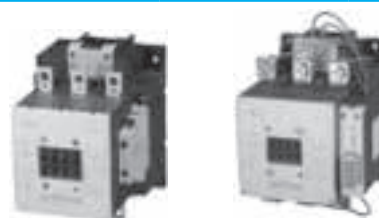
3RT1054-6A . . 6
