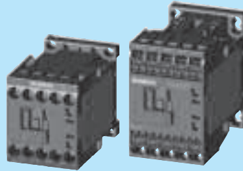
3RT13 / 23 contactors, AC-1: 18 to 140 A with 4 NO main contacts, sizes S00 to S3 with screw or spring connections
